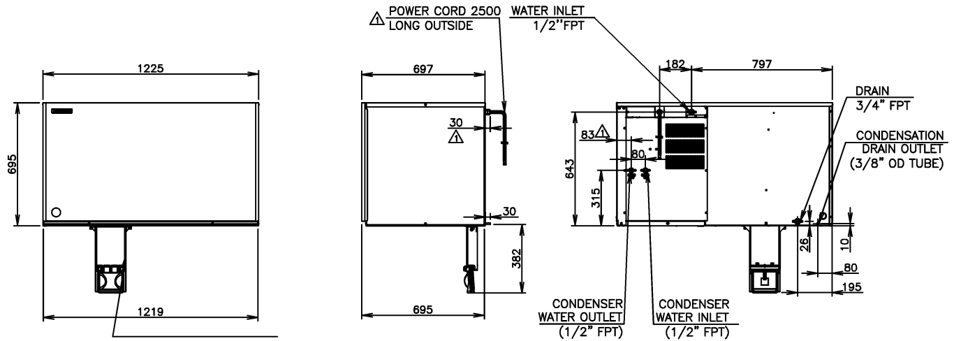
MECHANICAL BIN CONTROL (SHOWN INSTALLED)
