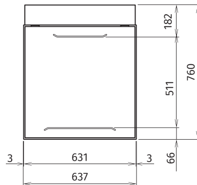
操作台布置 (直线)
